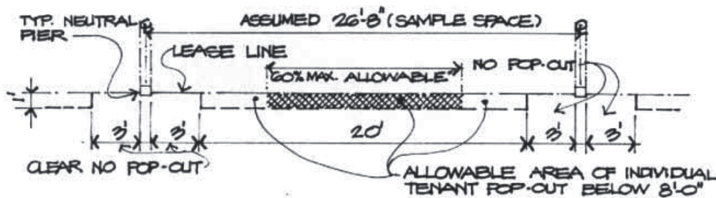
PLAN OF AN ASSUMED TENANT SPACE BELOW 8'0"
