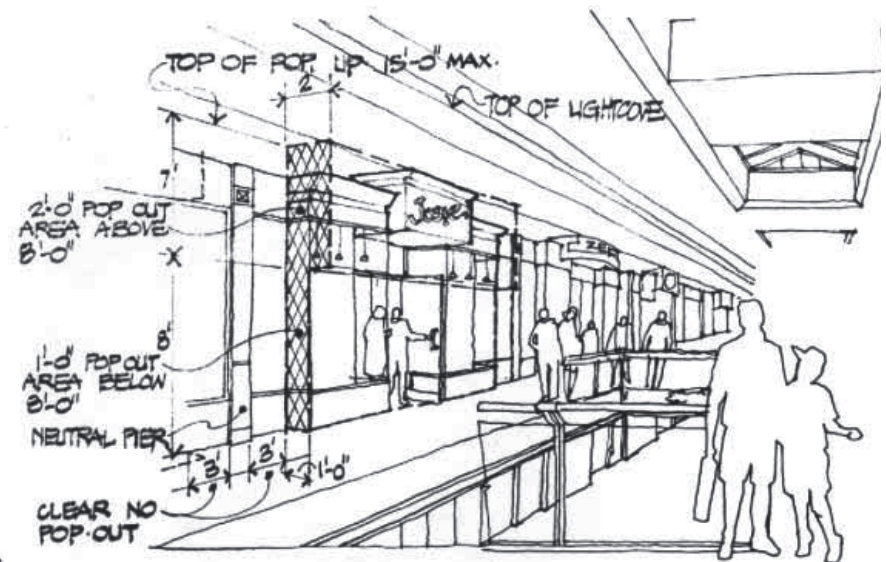
UPPER LEVEL POP-OUT
