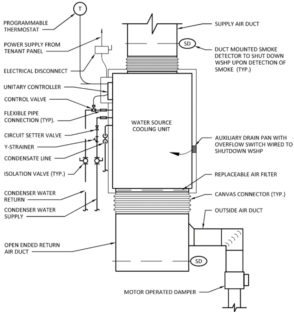
TENANT WATER SOURCE COOLING UNIT DETAIL
